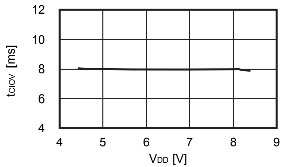
2.11 t_{\text{CI OV}} - V_{\text{DD}}
