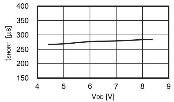
2.14 t_{\text{SH ORT}} - V_{\text{DD}}
