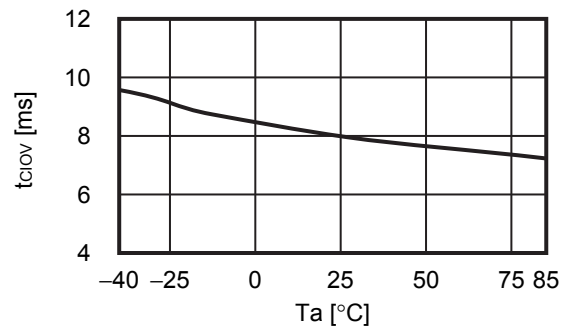
2.12 t_{\text{CI OV}} - T_a
