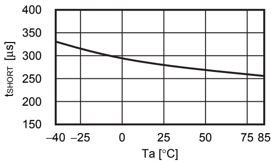
2.15 t_{\text{SH ORT}} - T_a
