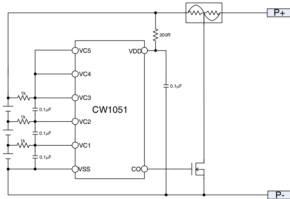
Reference Schematic for 3 cells
